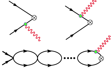
Figure 14: The leading order contribution to np \rightarrow d\gamma . Solid lines denote nucleons, wavy lines denote photons. The photon coupling is through the nucleon anomalous magnetic moment operator in \mathcal{L}_B ; the resummed unmarked vertex is the C_0 interaction. The crossed circle represents and insertion of the deuteron interpolating field \mathcal{D}_i . The bubble chain without photon insertions (not shown) is used to compute the wave function renormalization Z , and to fit C_0 to get the correction deuteron binding energy. See [17–19].
