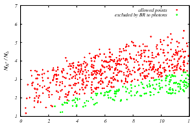
limits on \lambda_3 , M_H^\pm/M_h plane
